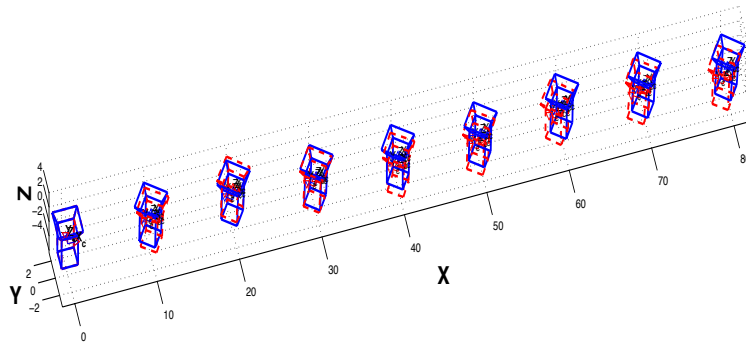
Figure 11: This figure shows the camera trajectory estimated from a sequence of images (see figure (9) for sample images). The camera frames drawn with solid (blue) lines depict the trajectory estimated using the Radon transform, while the dashed (red) lines show the RANSAC trajectory. In this sequence the motion is known to be approximately planar in the equatorial plane. Since the magnitude of camera motion cannot be recovered from pairs of images alone, we have fixed the distance between camera positions to be 10 units for visual purposes.
