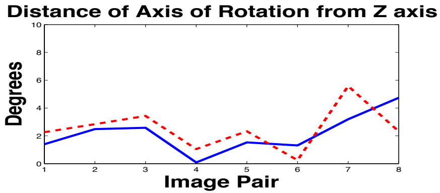
Figure 13: As the camera motion in this sequence (see figure (9) for sample images) is known to be roughly planar, we know that the axis of rotation must align with the Z axis. This plot shows for all eight image pairs in the sequence the distance in degrees of the estimated axis of rotation from the Z axis. The solid line (blue) is the estimate from our Radon integral, and the dashed line (red) is the RANSAC estimate.
