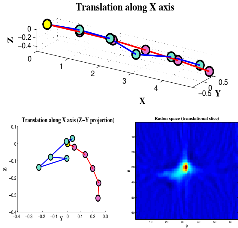
Figure 6: Top: the estimated trajectory of the camera. In blue (light) is the Radon estimation, in red (dark) is the RANSAC computation, and the yellow circle marks the starting position. Bottom Left: A projection of the trajectory onto the Z-Y plane showing the deviation of the estimated positions from the X axis. Bottom Right: the R_t slice of the grid G where the maxima was found.
