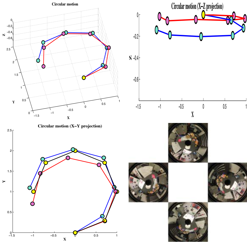
Figure 8: A camera moving along a circular path. Top Left: In blue (light) is the Radon estimation, in red (dark) is the RANSAC. Top Right: A projection onto the X-Z plane showing the deviation from the plane of the turntable. Bottom Left: An overhead view. The yellow circles are the observed ground truth positions of the camera. Bottom Right: four images from the sequence. Even though the dominant motion is rotation, the translation is still effectively detected by the Radon.
