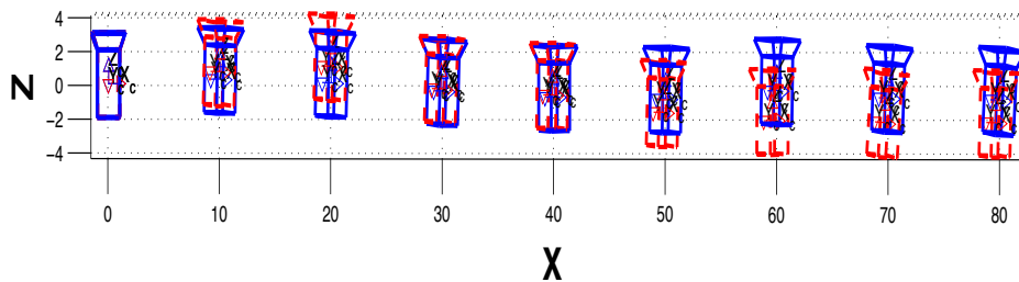
Figure 12: This figure shows the camera trajectory estimated from a sequence of images (see figure (9) for sample images), projected onto the ZX plane. The camera frames drawn with solid (blue) lines depict the trajectory estimated using the Radon transform, while the dashed (red) lines show the RANSAC trajectory. The motion is known to be planar (on the equatorial plane) and the Radon estimate reflects this more accurately. Since the magnitude of camera motion cannot be recovered from images alone, we have set the distance between camera positions to be 10 units for visual purposes.
