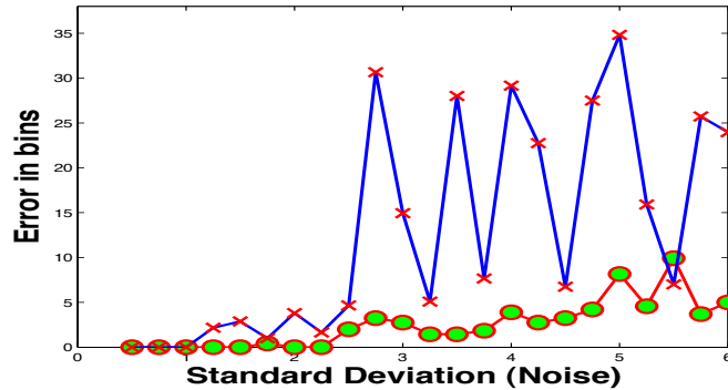
Figure 4: Results of a simulation testing the robust accumulation in the presence of Gaussian noise. The locations of spherical point correspondences are perturbed with Gaussian noise in each spherical coordinate. The standard deviation of the noise distribution is given here in pixels, and the error is computed by measuring the distance of the estimated solution from the correct solution in the 5D motion space. The plot marked with 'x' represents the simulation performed with bandwidth L = 24 . In this case, a standard deviation of one pixel corresponds to 7.5^\circ and 3.8^\circ in the spherical coordinates \phi and \theta . The plot marked with circles is for L = 32 , where a standard deviation of one pixel corresponds to 5.6^\circ and 2.8^\circ in the spherical coordinates. For this higher bandwidth, the results are still accurate in presence of significant noise.
